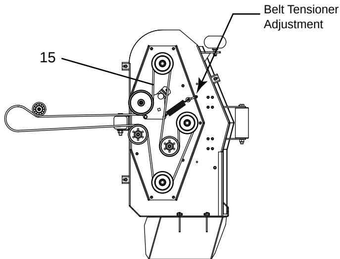
VIEWS FROM UNDER OF DECK
