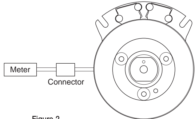
Figure 2 Voltage Measurement
