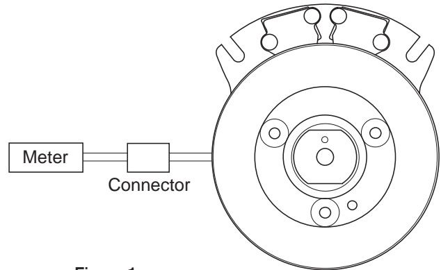
Figure 1 Resistance Measurement
